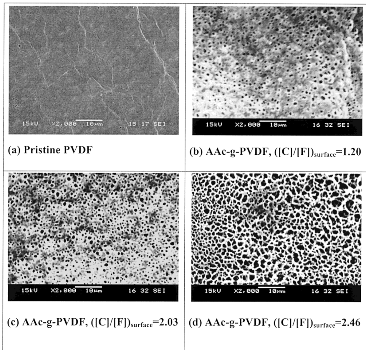
Figure 5. SEM micrographs of the MF membranes cast with phase inversion from 12% (w/w) NMP solutions of (a) the pristine PVDF and the AAc-g-PVDF copolymers of graft concentrations ( ([C]/[F])_{\text{surface}} ratios) of (b) 1.20, (c) 2.03, and (d) 2.46.
