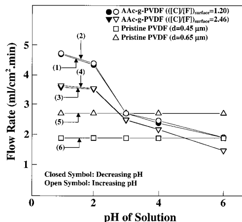
Figure 8. pH-dependent water permeability through the AAC-g-PVDF and the pristine PVDF MF membranes. Curves 1 and 2 and curves 3 and 4 are obtained on two AAC-g-PVDF MF membranes of different graft concentrations when subjected to pH cycling, while curves 5 and 6 are the flux through the commercial PVDF membranes (standard pore size, d = 0.65 \mu\text{m} and d = 0.45 \mu\text{m} , respectively) with characteristic pore size distributions similar to those of the AAC-g-PVDF copolymer membranes.
