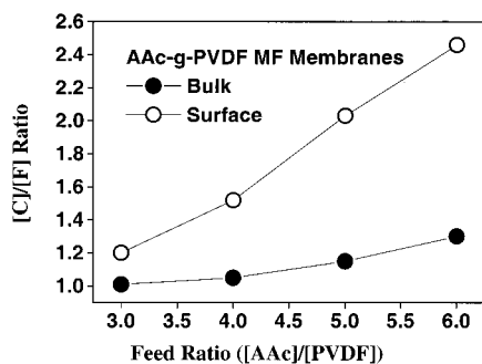
Figure 7. Comparison between surface and bulk graft concentration of the MF membranes cast via the phase inversion from 12% (w/w) NMP solutions of the AAC-g-PVDF copolymers of different graft concentrations.
